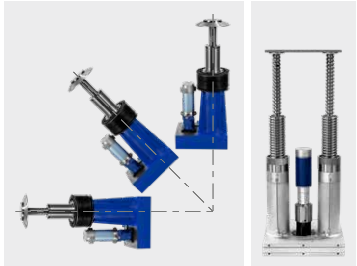
Telescopic actuators for all mounting positions
